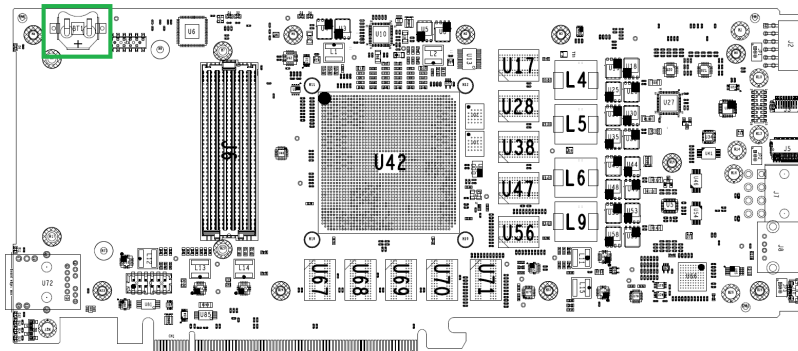
Figure 20 : Battery Location
