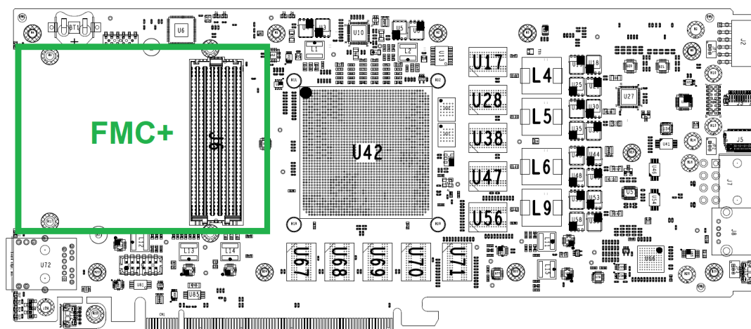
Figure 12 : FMC+ Location
