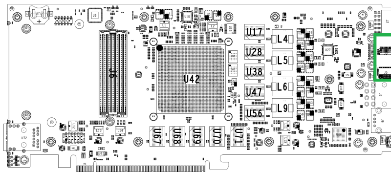
Figure 14 : FireFly Locations
